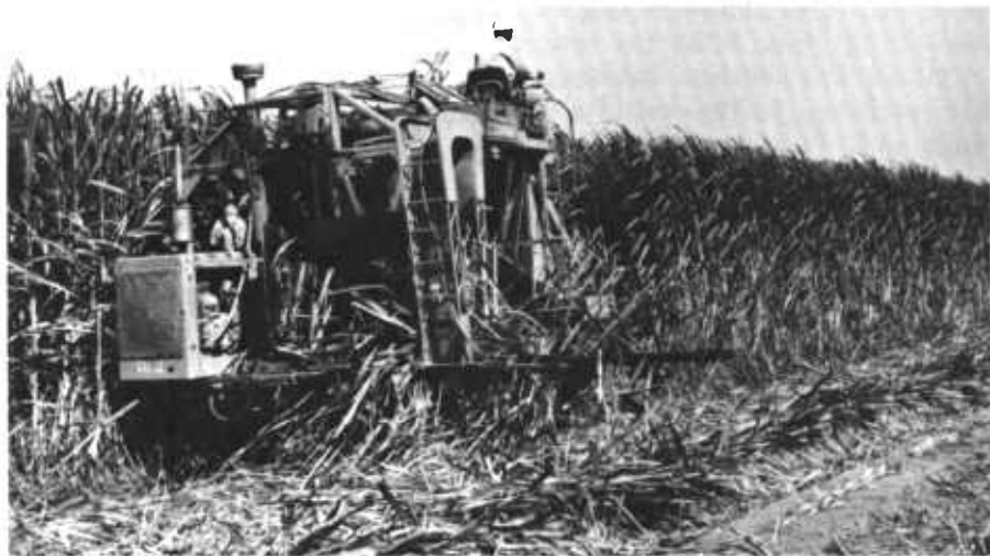
Figure 21.—Sugarcane harvester cutting sugarcane.
