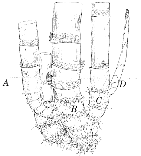
Figure 6.—Diagram of part of a sugarcane stool: A , Ground level; B , primary; C , secondary; and D , tertiary shoots. (After Artschwager.)
